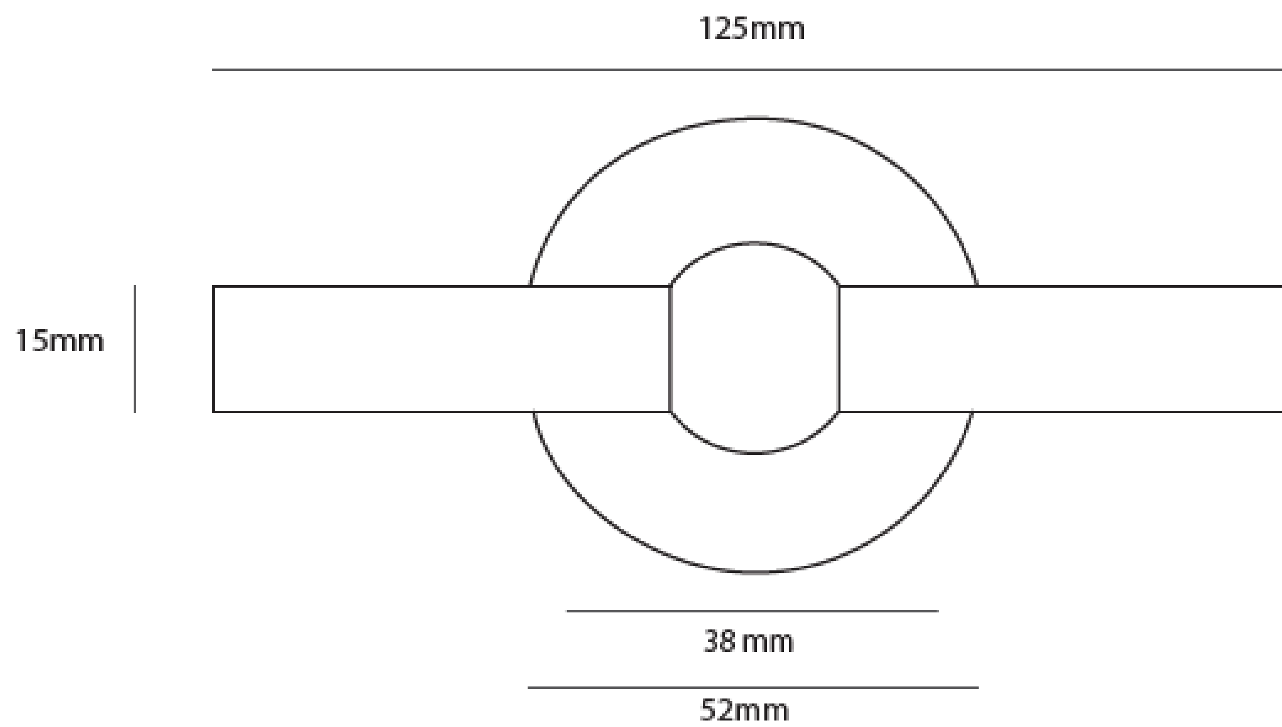
Top view
