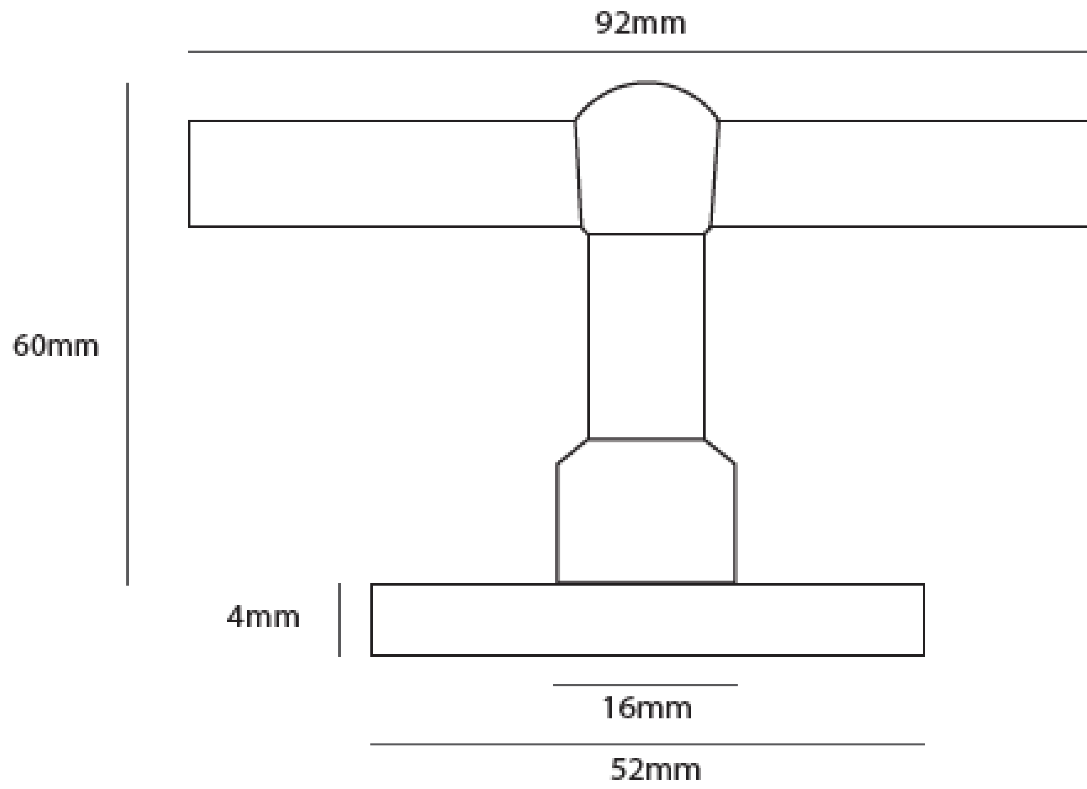
Side view
