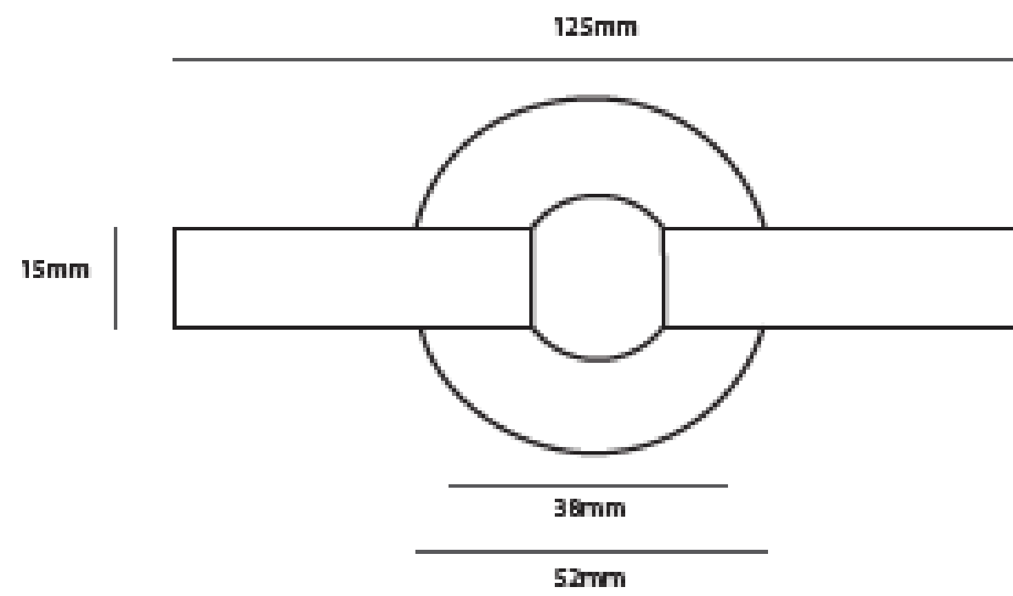
Top view
