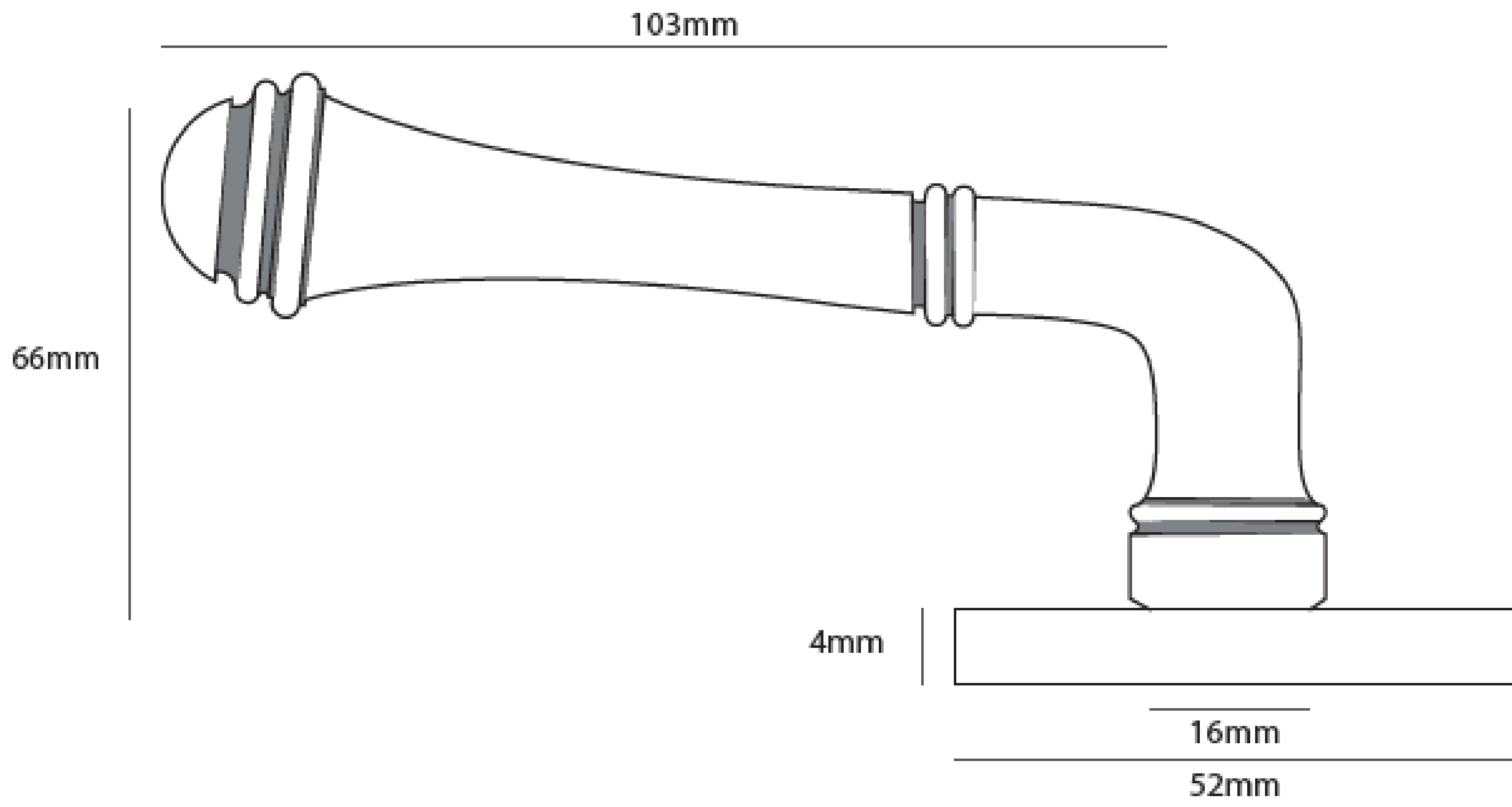
Side view
