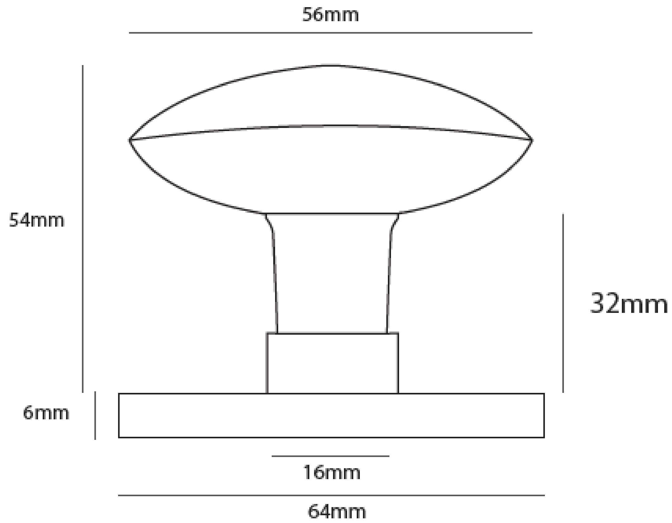
Side view
