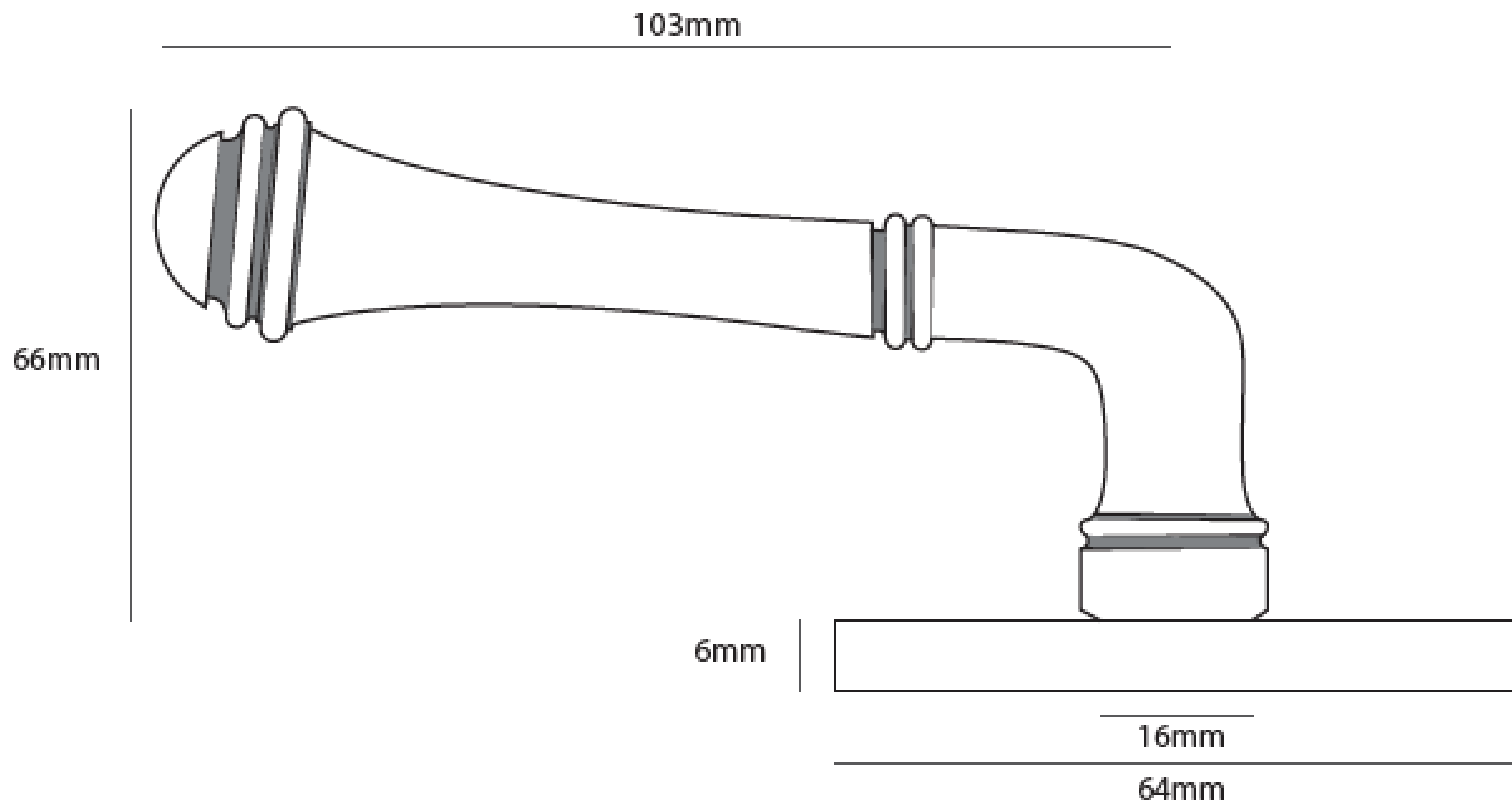
Side view
