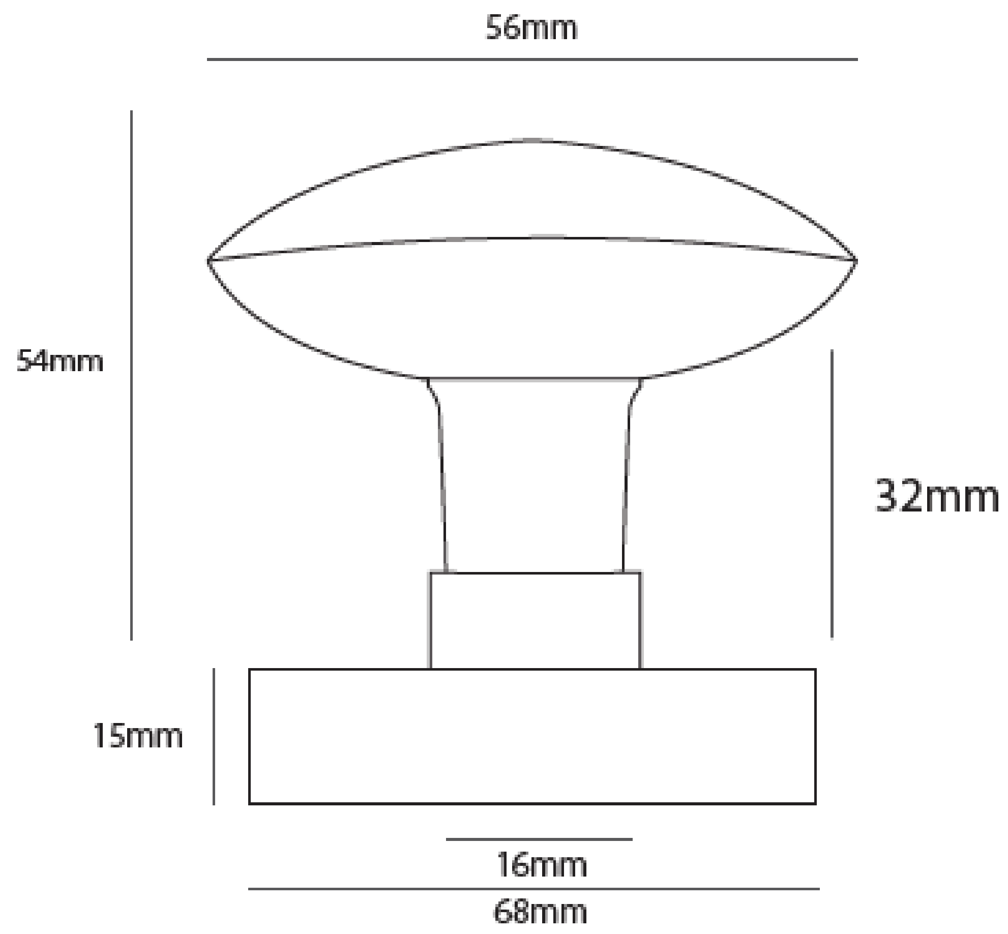
Side view
